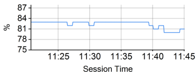
Humidity
