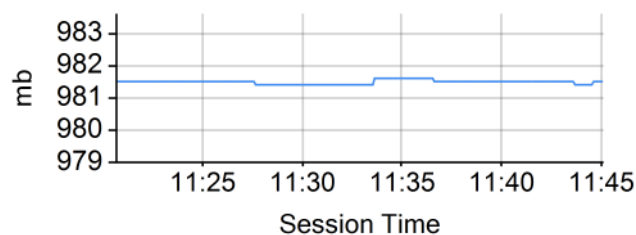
Barometric Pressure
