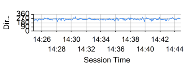
Wind Direction
