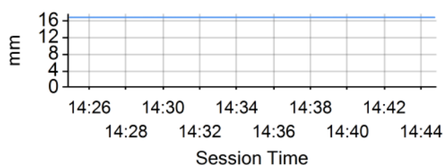
Daily Rainfall
