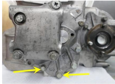
'Sealing 9' – Speedo drive/Gearbox end casing
